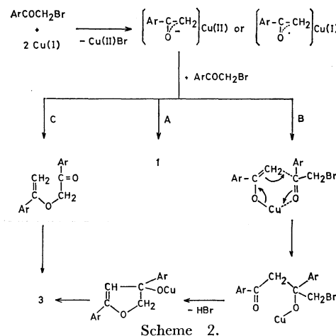
Scheme 2.
